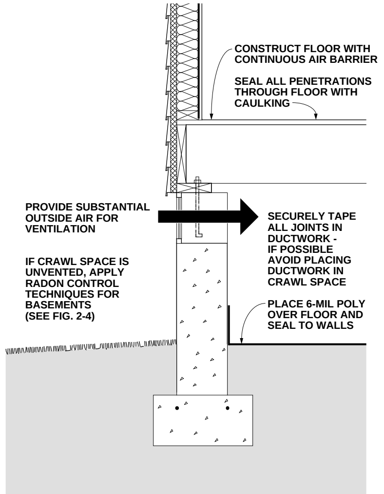
Figure 3-6: Radon Control Techniques for Crawl Spaces
