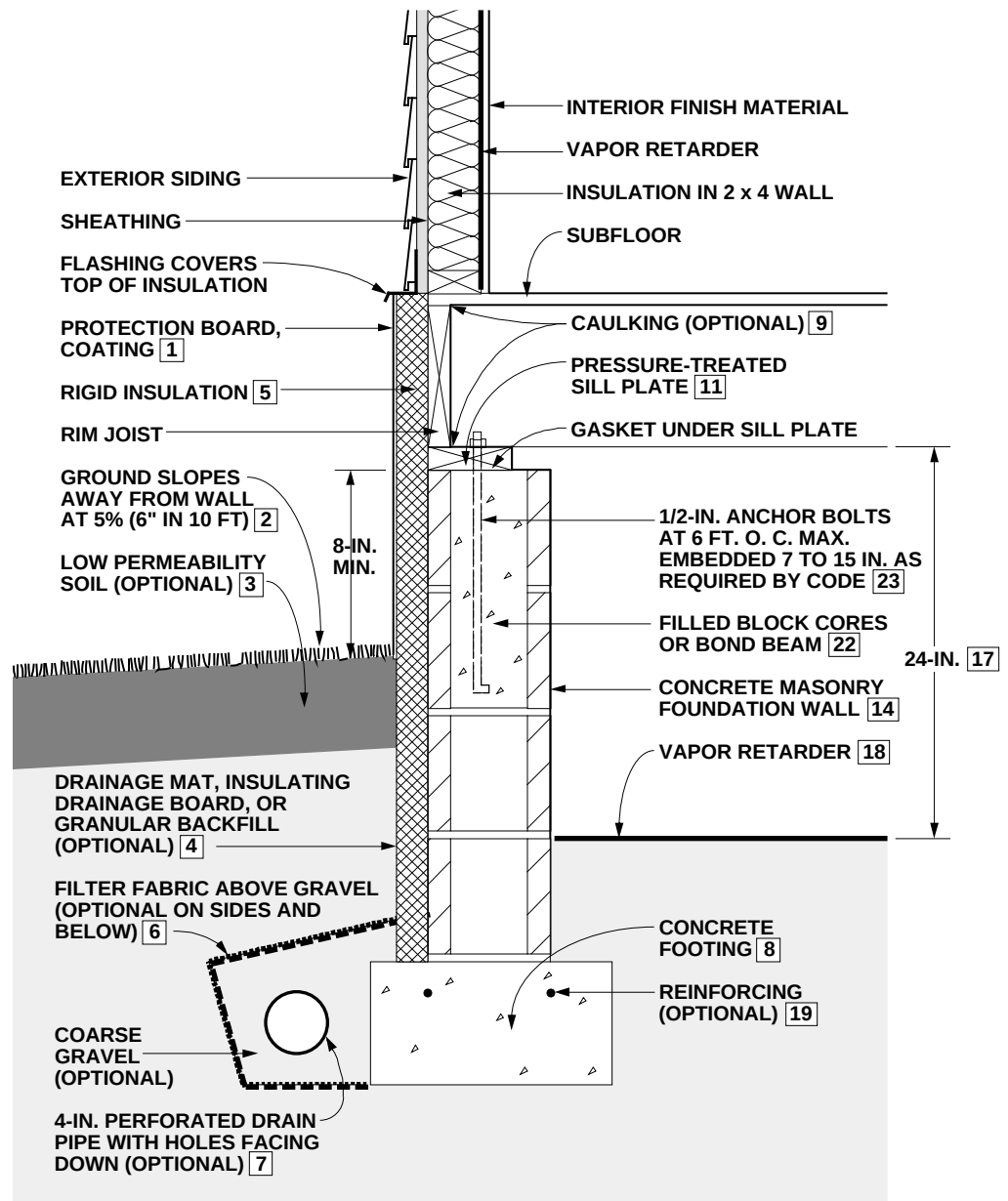
Figure 3-9: Unvented Crawl Space Wall with Exterior Insulation
